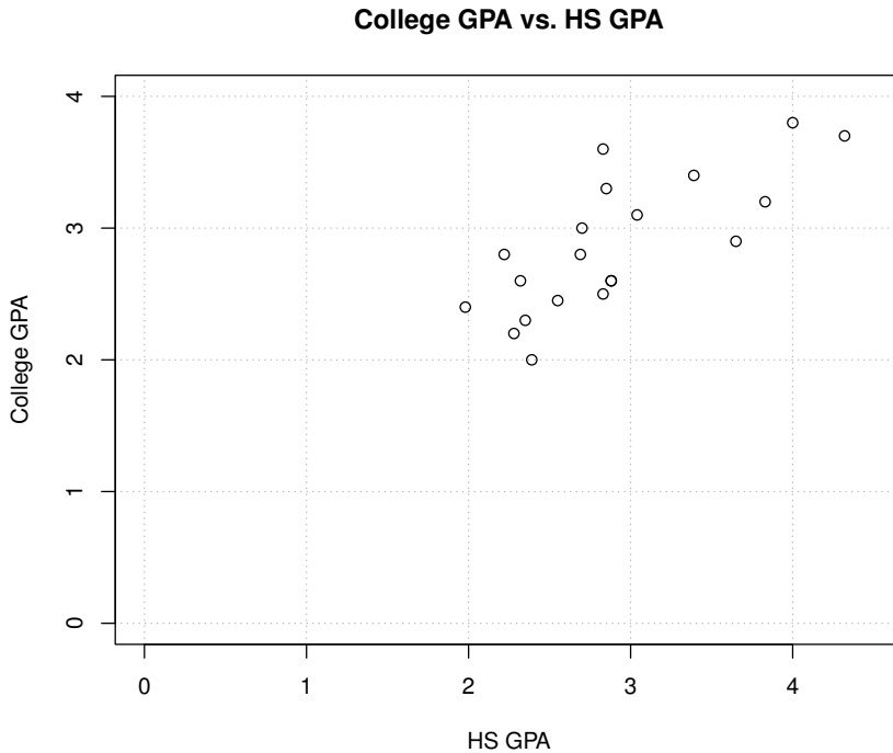
Figure A.7: Scatter plot using optional arguments.
