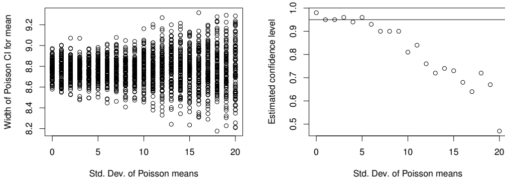
Figure 5.5: Likelihood ratio confidence interval results from simulations using overdispersed Poisson data. Confidence interval widths (left) and estimated confidence levels (right) are plotted against the standard deviation of the means used to generate the Poisson data. The horizontal line in the confidence level plot shows the stated confidence level of 95%.
