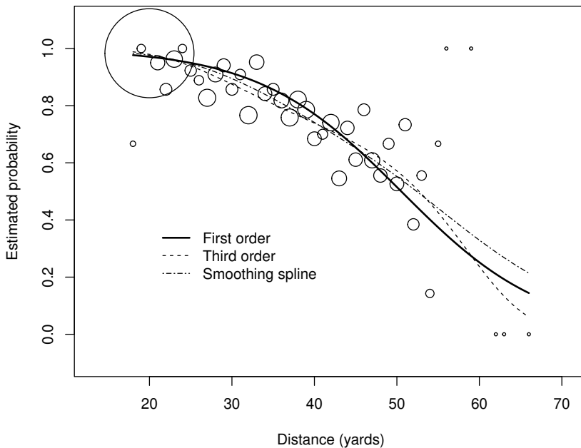
Figure 6.18: Smoothing spline model compared to first- and third-order models for the placekick data.
