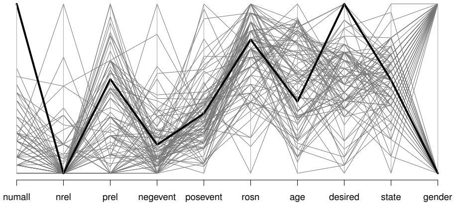
Figure 5.17: Parallel coordinate plot highlighting observation 58's position relative to the rest of the data.
