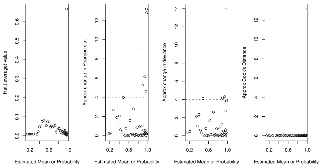
Figure 5.3: Plots of influence measures vs. estimated probabilities of success for the placekicking data. Dotted lines represent thresholds for potentially high influence.
