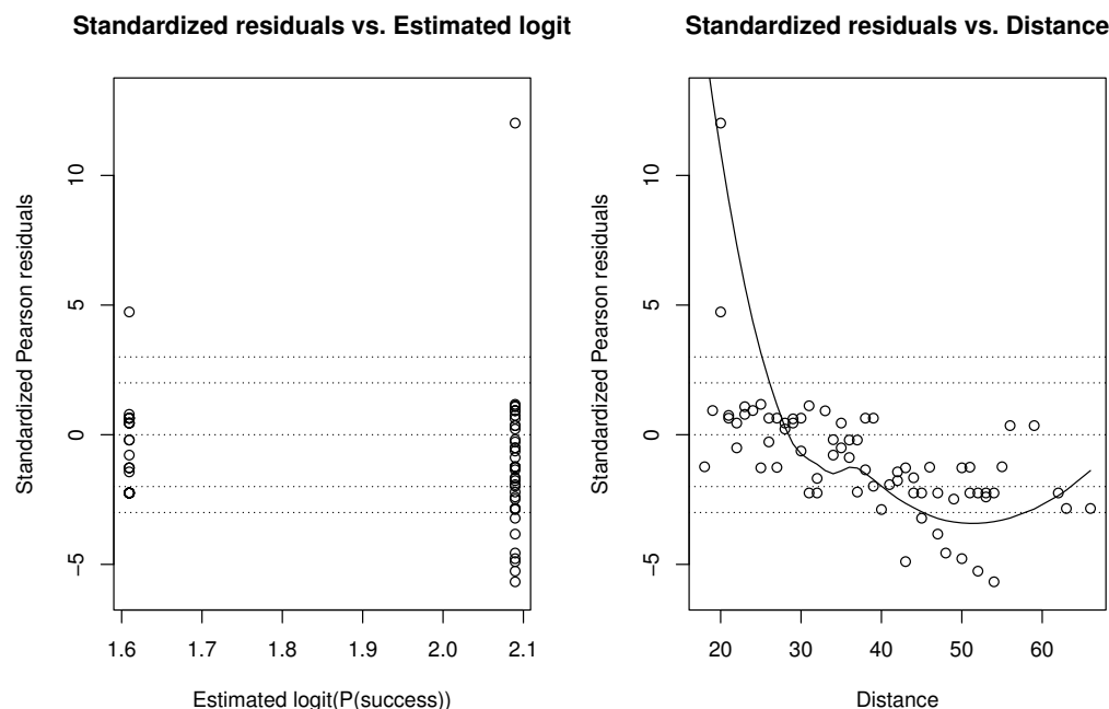
Figure 5.7: Standardized residual plots for placekick data when the logistic regression model contains only wind. Lines at \pm 2 and \pm 3 are approximate thresholds for standardized residuals. Left: Residuals versus the logit of the estimated probability of success. Right: Residuals versus the omitted variable distance , with the curve from a weighted loess smoother added to accentuate the mean trend.
