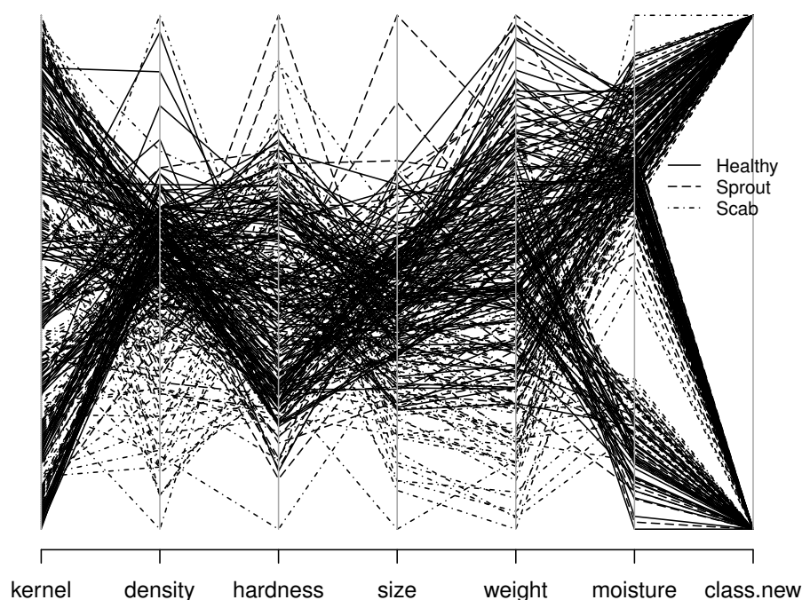
Figure 3.2: Parallel coordinate plot of the wheat data. The kernel variable corresponds to the observation number in the data set. The class.new variable is a 1 for soft red winter wheat and 0 for hard red winter wheat. We recommend viewing this plot in color (see program for code) if the version in your book is only in black and white.
