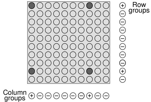
Figure 6.14: Diagram of group testing performed in a two dimensional array-like structure. Filled-in circles indicate which specimens need to be retested because of positive row and column tests. Reproduced by permission of Christopher R. Bilder.
