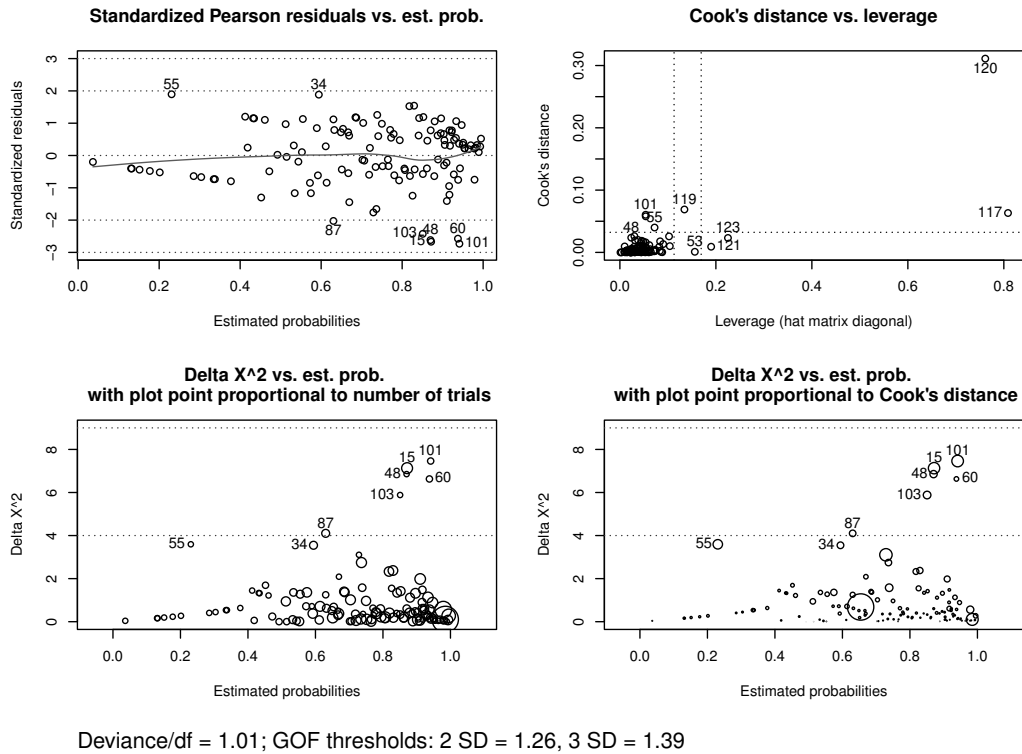
Figure 5.11: Diagnostic plots for the placekicking logistic regression model; all observations are included in the data set.
