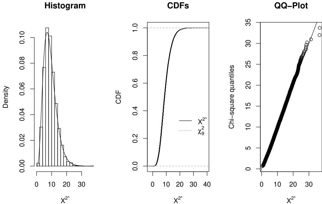
Figure 3.1: Plots of X^{2*} and a \chi^2_9 distribution.
