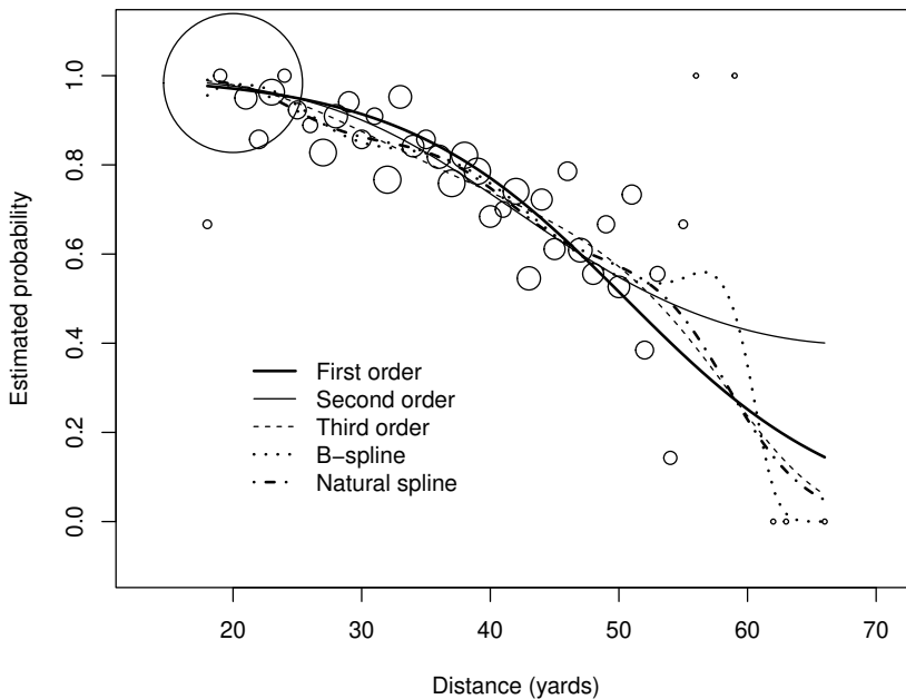
Figure 6.16: Spline models compared to first-, second-, and third-order models for the placekick data.
