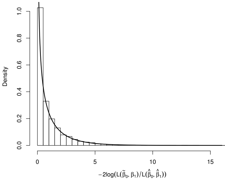
Figure 2.11: Histogram of -2\log(\Lambda) with \chi^2_1 distribution overlay.
