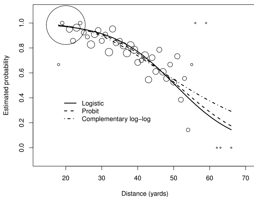
Figure 2.14: Bubble plot of the estimated probability of success for a placekick. The observed proportion of successes at each distance is plotted with the plotting point size proportional to the number of observations at a distance. The estimated logistic, probit, and complementary log-log regression models are all given in the plot.
