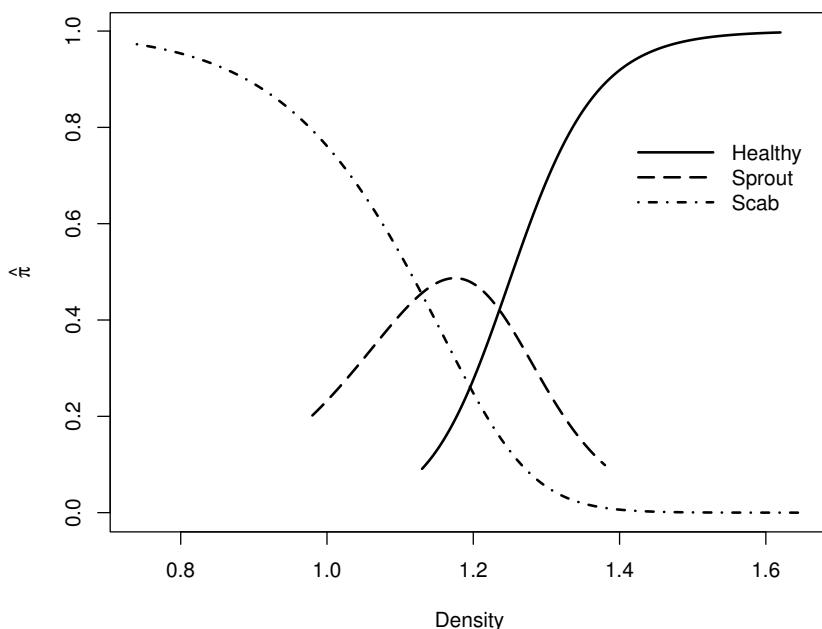
Figure 3.3: Estimated multinomial regression model for the wheat data with density as the only explanatory variable in the model.
