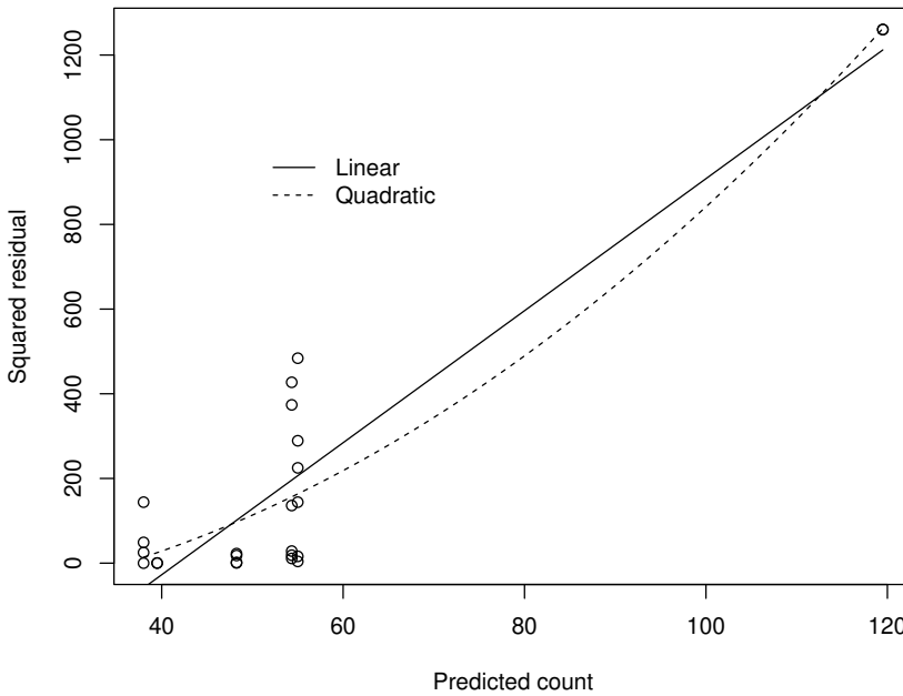
Figure 5.9: Plot of squared residuals vs. predicted values for choosing between quasi-Poisson and negative binomial models. Solid line is the straight line fit for quasi-Poisson model; dashed line is quadratic fit for negative binomial.
