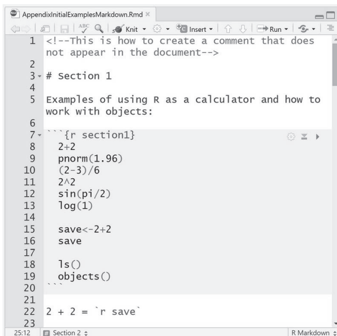
Figure A.4: Screen capture of using R Markdown in RStudio.
