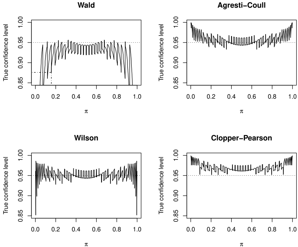
Figure 1.3: True confidence levels with n = 40 and \alpha = 0.05 . The Wald plot includes a dot-dashed line illustrating that the true confidence level is 0.8760 at \pi = 0.157 .
