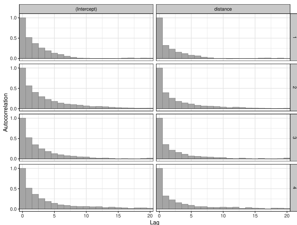
Figure 6.12: Bar plots of the autocorrelations for each chain.
