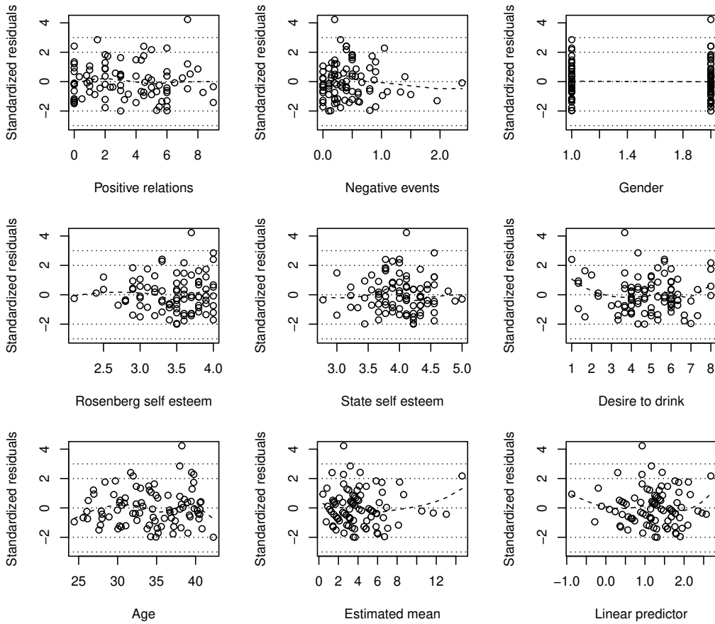
Figure 5.15: Residual plots from the working Poisson regression model for the alcohol consumption data.
