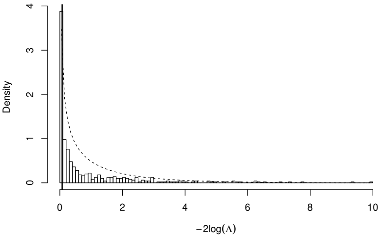
Figure 6.8: Histogram of LRT statistics using parametric resampling under H_0 : \sigma^2_{b0} = 0 for the falls example. The histogram excludes 500 resamples with LRT statistic values of zero that are expected to occur by chance under H_0 . The thick vertical line indicates the location of the statistic from the original data. The dashed curve is the \chi^2_1 approximation.
