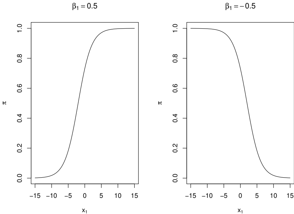
Figure 2.1: Logistic regression model for \beta_0 = 1 and \beta_1 = 0.5 and -0.5 .
