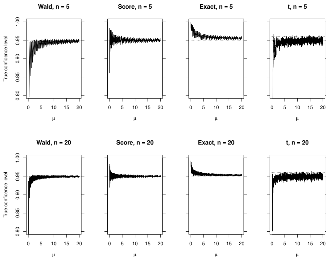
Figure 4.2: True confidence level for Wald, score, and exact 95% confidence intervals and estimated true confidence level for 95% t -based interval. The dotted line at 0.95 represents the stated level; additional horizontal lines in t -based interval plot are limits within which the estimated true confidence levels should fall 95% of the time if the true confidence level is 0.95.
