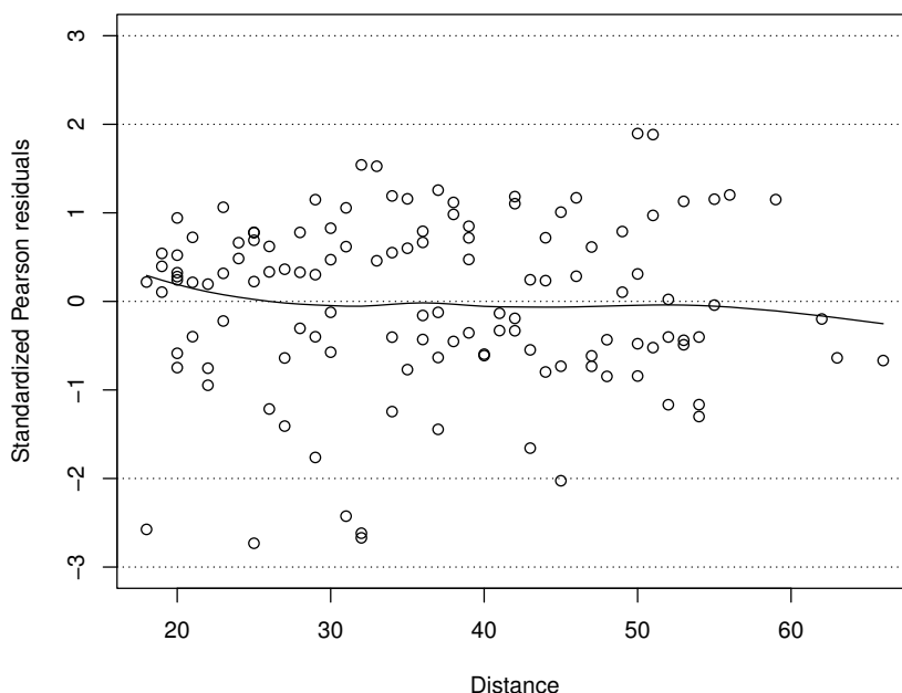
Figure 5.10: Standardized Pearson residuals vs. distance of the placekick.
