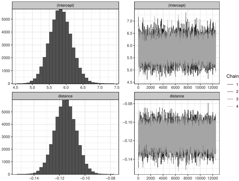
Figure 6.11: Histograms and trace plots for the \beta_0 and \beta_1 sampled values.
