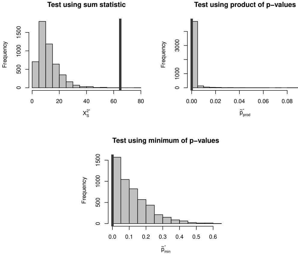
Figure 6.4: Histograms of the estimated probability distributions under SPMI. The vertical lines denote the observed statistic value for the original data.
