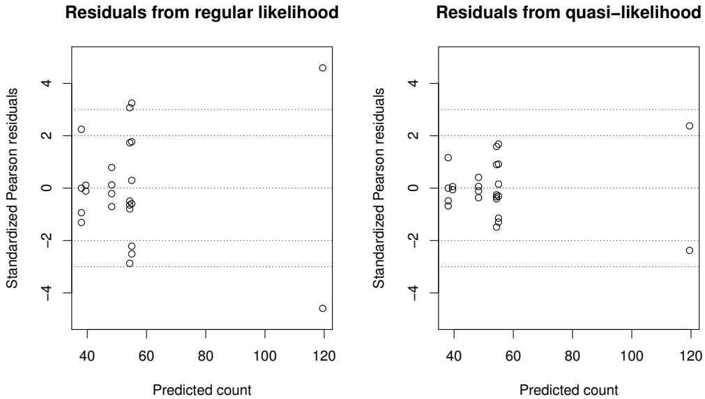
Figure 5.6: Standardized residuals plotted against the mean for the Ecuadorean bird count data. Left: Residuals from the fit of the original Poisson model. Right: Residuals from the fit of a quasi-Poisson model. In both cases, upper and lower dotted lines are given at \pm 2 and \pm 3 to aid interpretation of the plots.
