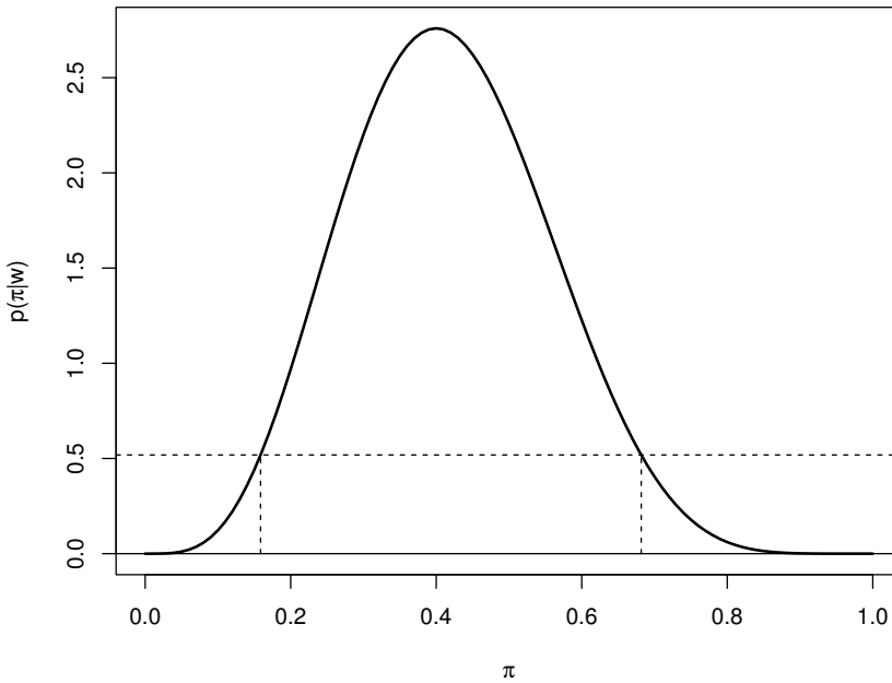
Figure 6.10: Posterior density plot with a horizontal line drawn at p(\pi|w) = 0.5184 and vertical lines indicating the limits for the 95% HPD interval.
