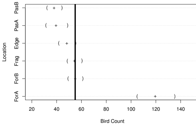
Figure 4.7: Plot of MLEs for mean bird counts, denoted by “+”, and LR confidence intervals, denoted by parentheses, for mist-netted bird captures at six locations in Ecuador. The vertical line represents the overall mean of all counts.
