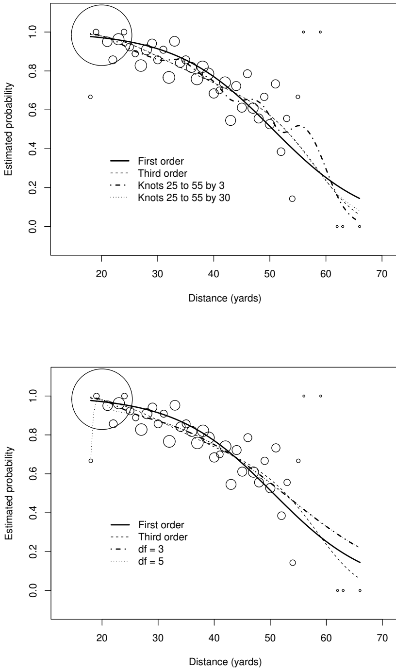
Figure 6.17: Natural spline models for a specified set of knots or a specified degrees of freedom when fit to the placekicking data. It is difficult to view the 5 degrees of freedom spline model for distances of 29 yards or larger because its fit is very close to the 3 degrees of freedom spline model.
