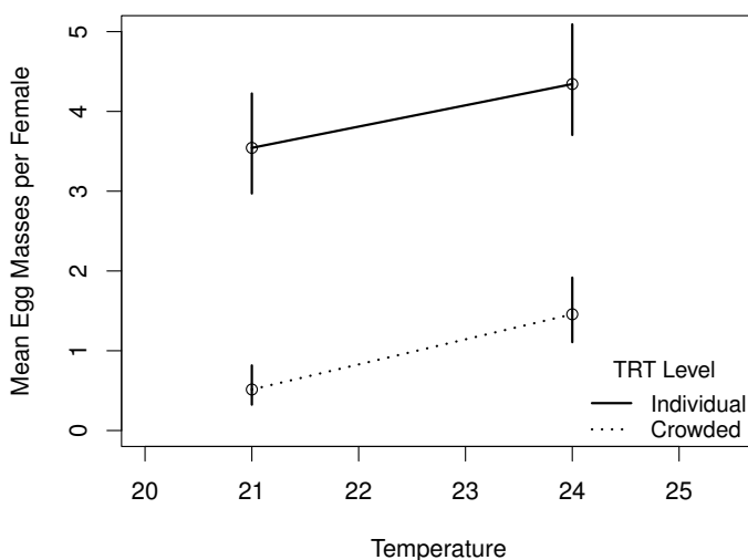
Figure 4.8: Estimated rates of egg mass production and confidence intervals for all treatment-temperature combinations in the beetle egg-laying example. Individual cages have one female and male; crowded cages have five females and males. The vertical lines represent 95% Wald confidence intervals for the rate.
