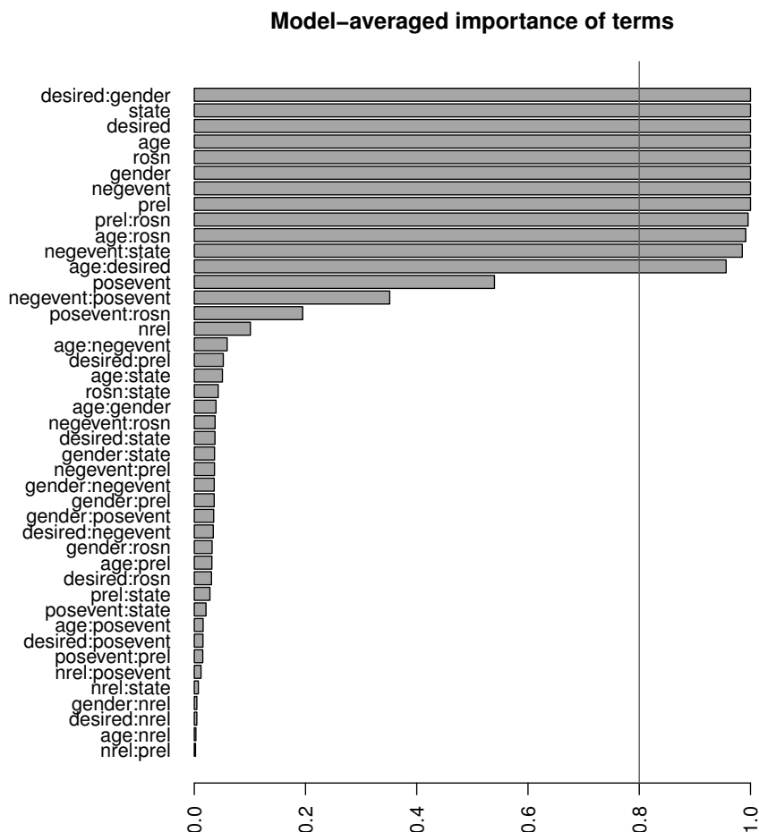
Figure 5.14: Results of genetic algorithm variable search for the alcohol consumption example using model averaging with evidence weights on all variables and two-way interactions.
