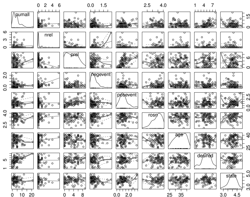
Figure 5.13: Scatterplot matrix of response ( numall ) and explanatory variables for alcohol consumption data.
