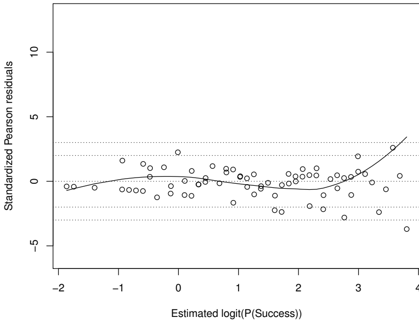
Figure 5.8: Standardized residuals against linear predictor for placekick data when the logistic regression model for success contains wind speed and distance. Upper and lower lines at \pm 2 and \pm 3 are approximate thresholds for standardized residuals. The solid curve is from a weighted loess smoother to highlight any mean trend.
