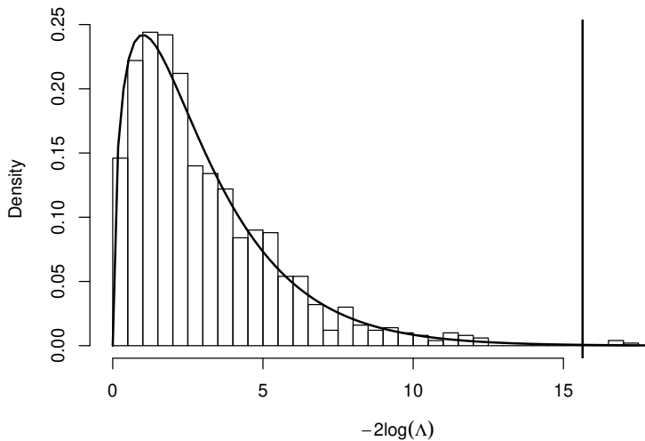
Figure 6.6: Comparison of parametric bootstrap estimate of the distribution of -2\log(\Lambda) with the large-sample \chi^2_3 distribution. The vertical line marks the value of the -2\log(\Lambda) in the original data.
