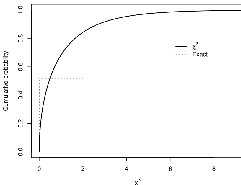
Figure 6.1: Exact and chi-square CDFs for tea-tasting example.
