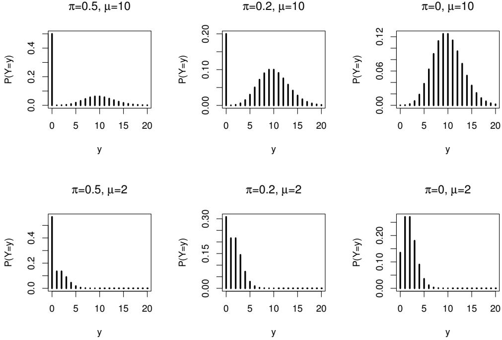
Figure 4.9: Probability mass histograms from zero-inflated Poisson models with varying means and levels of zero inflation. These plots are created by ZeroInflPoiDistPlots.R .
