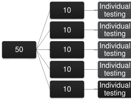
Figure 6.13: Diagram of group testing performed over three hierarchical stages. Reproduced by permission of Christopher R. Bilder.
