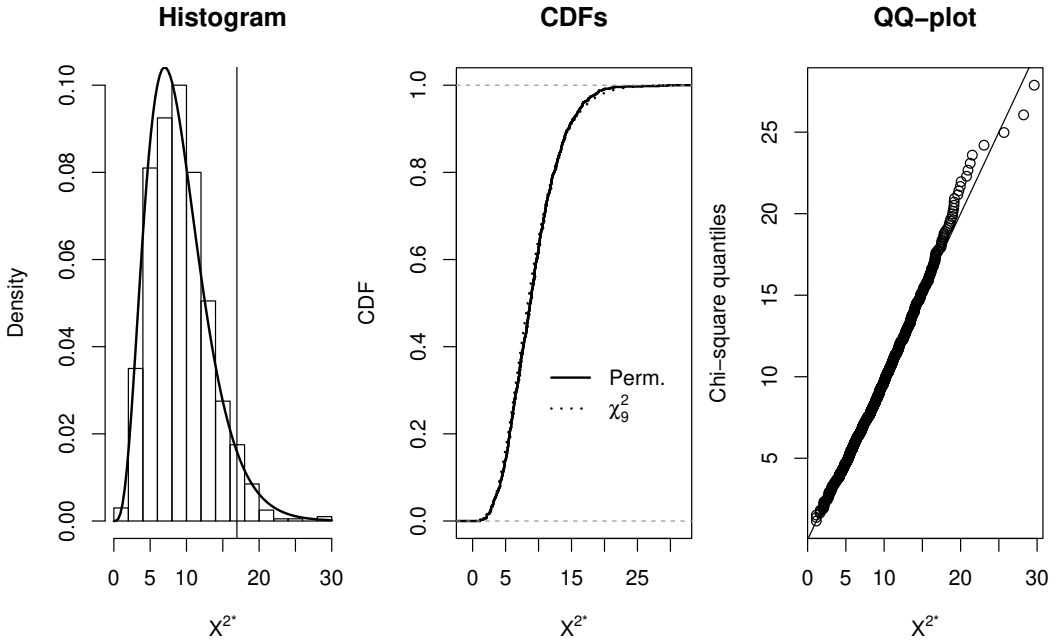
Figure 6.2: Permutation and chi-square distributions. The vertical line in the histogram is drawn at X^2 = 16.94 .
