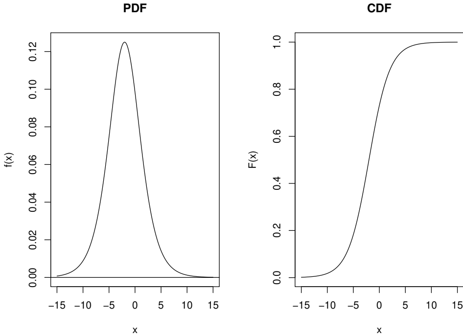
Figure 2.12: PDF and CDF for the logistic probability distribution with \mu = -2 and \sigma = 2 .
