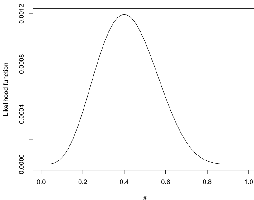
Figure B.1: Bernoulli likelihood function evaluated at w = 4 and n = 10 .
