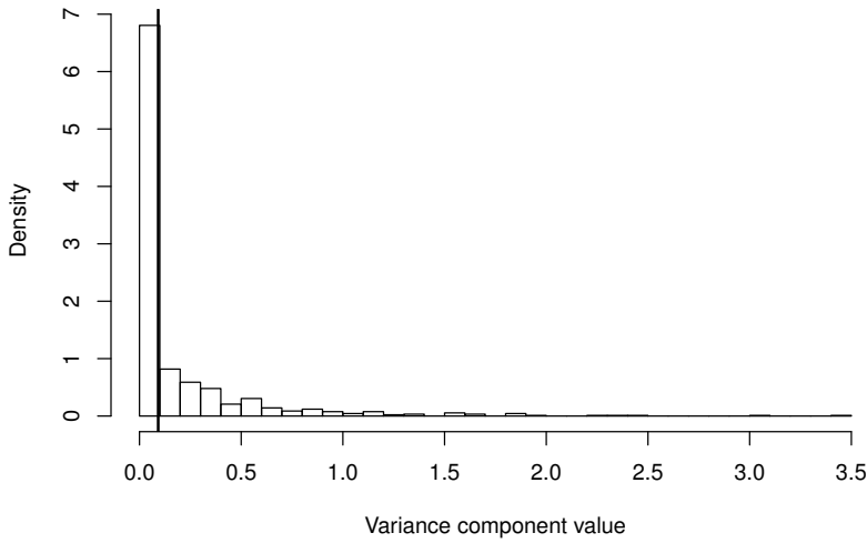
Figure 6.7: Histogram of variance component estimates using parametric resampling under H_0 : \sigma_{b0}^2 = 0 for the falls example. The thick vertical line indicates the location of the estimate from the original data.
