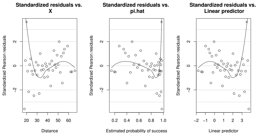
Figure 5.2: Residual plots for modeling of the probability of success vs. distance.
