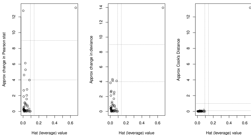
Figure 5.4: Plots of influence measures vs. leverage values for the placekicking data. Dotted lines represent thresholds for potentially high influence.
