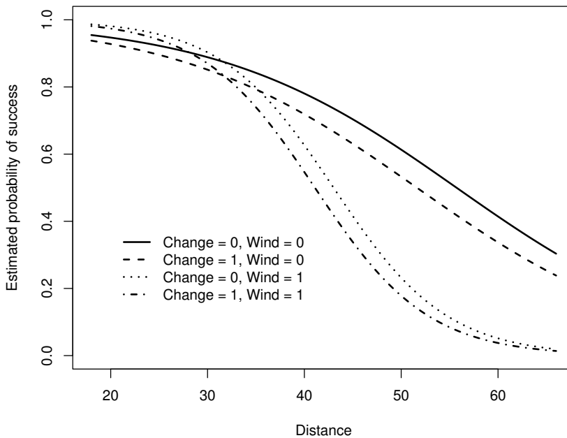
Figure 5.12: Estimated probability of success vs. the field goal ( PAT = 0 ) distance for four combinations of change and wind.
