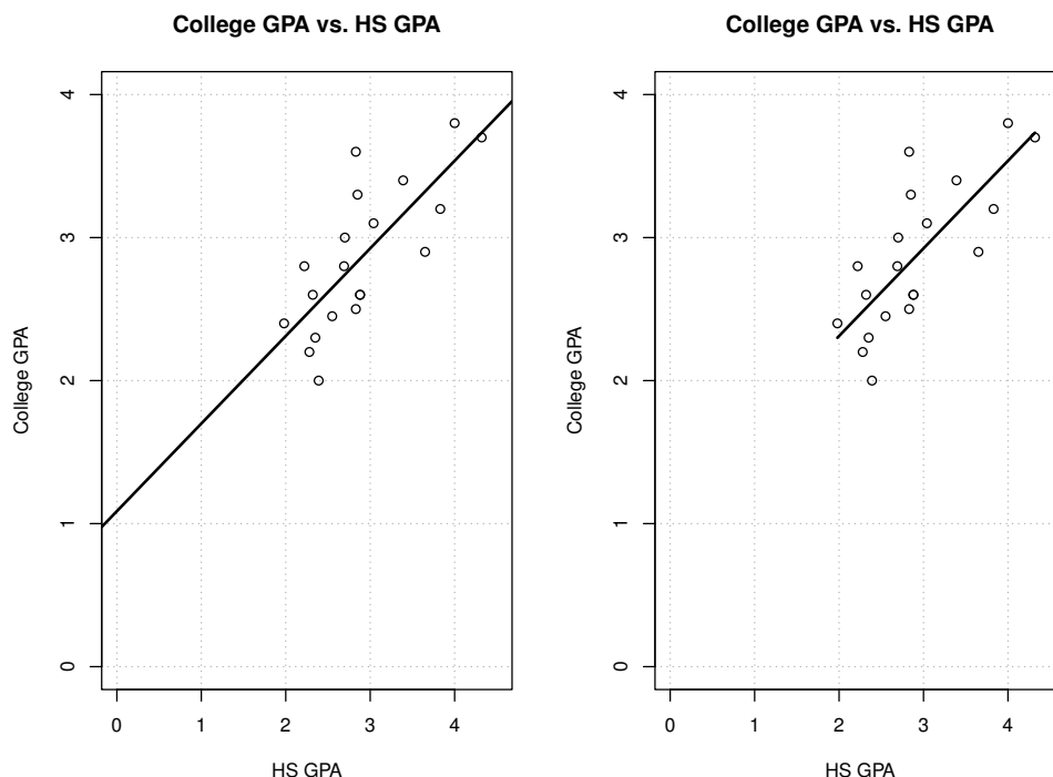
Figure A.8: Scatter plots with estimated model drawn using the abline() function (left) and curve() function (right).
