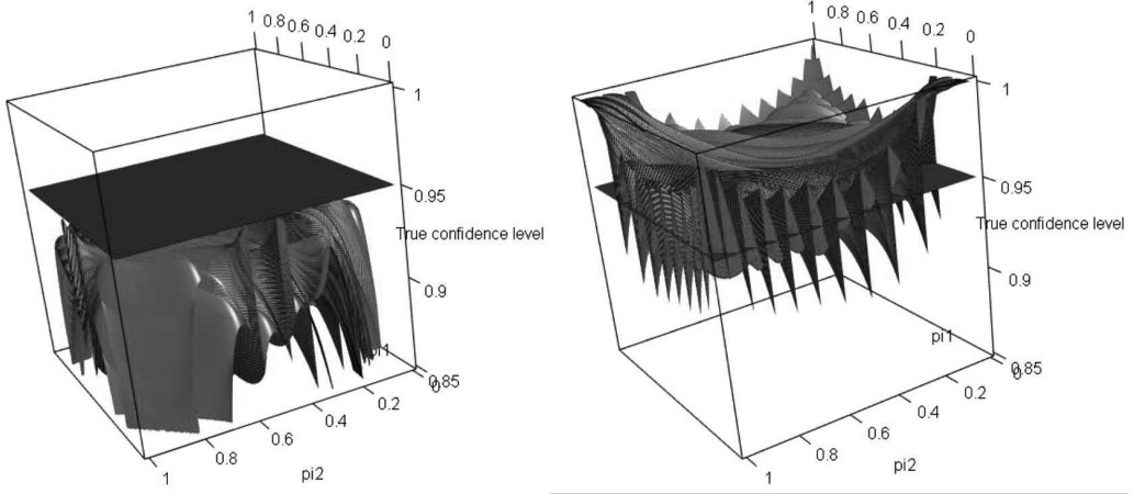
Figure 1.5: True confidence levels with n_1 = 10 , n_2 = 10 , and \alpha = 0.05 . The left plot is for the Wald interval, and the right plot is for the Agresti-Caffo interval. Note that true confidence levels less than 0.85 are excluded from the Wald interval plot.
