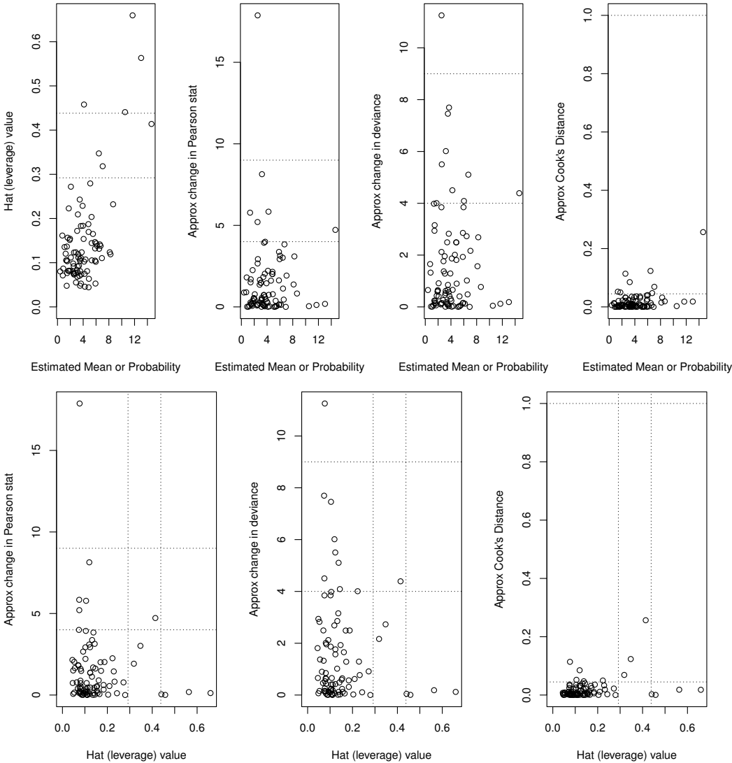
Figure 5.16: Influence diagnostic plots for alcohol consumption data.
