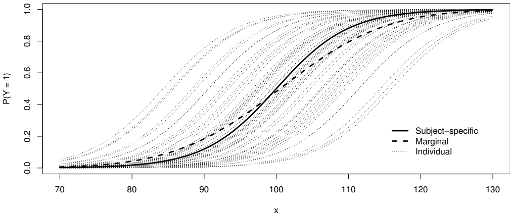
Figure 6.9: Subject-specific model and marginal model for simulated sample of 50 subjects from a population with probability of success following a logistic curve with common slope but different intercepts. The code to produce the plot is in LogisticSim.R .
