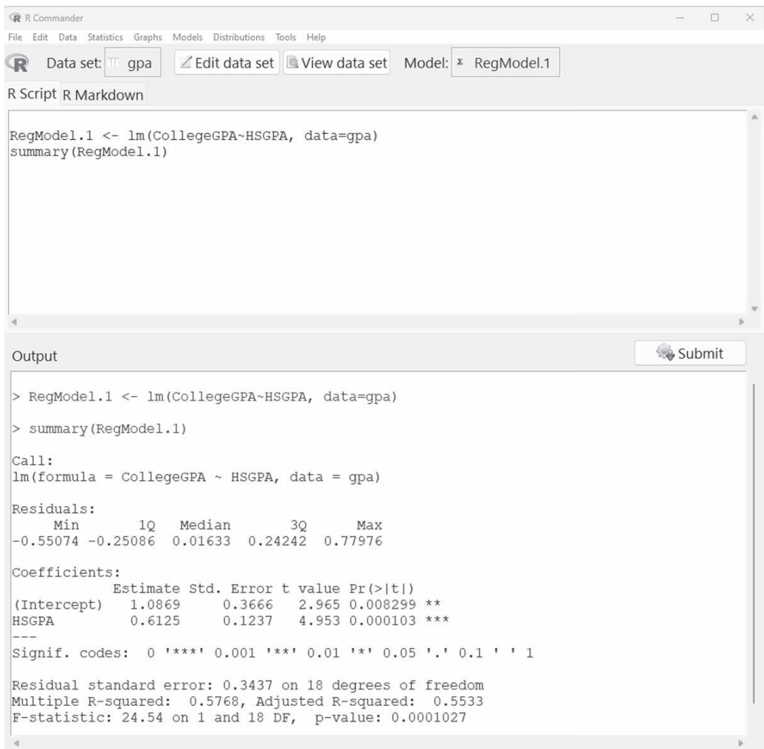
Figure A.10: R Commander window.
